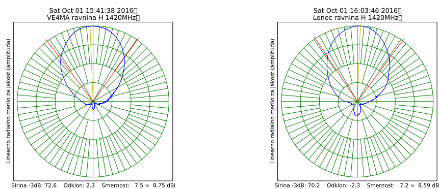
(a) Žarilec z obodom ovratnikom VE4MA
