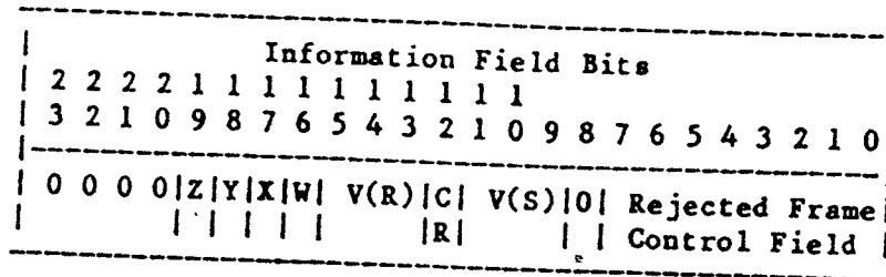
Fig. 9 — FRMR frame information field
