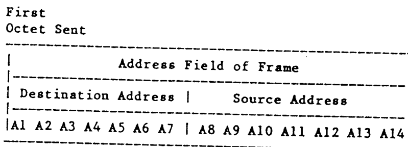
Fig. 2 -- Nonrepeater Address-Field Encoding
