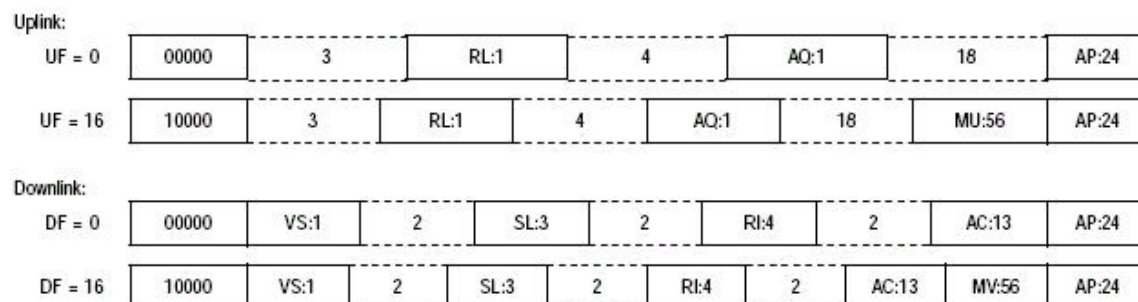
Figure 4-1. Surveillance and communication formats used by ACAS
