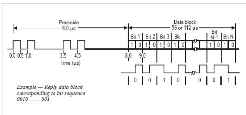
Figure 3-6. Mode S reply
