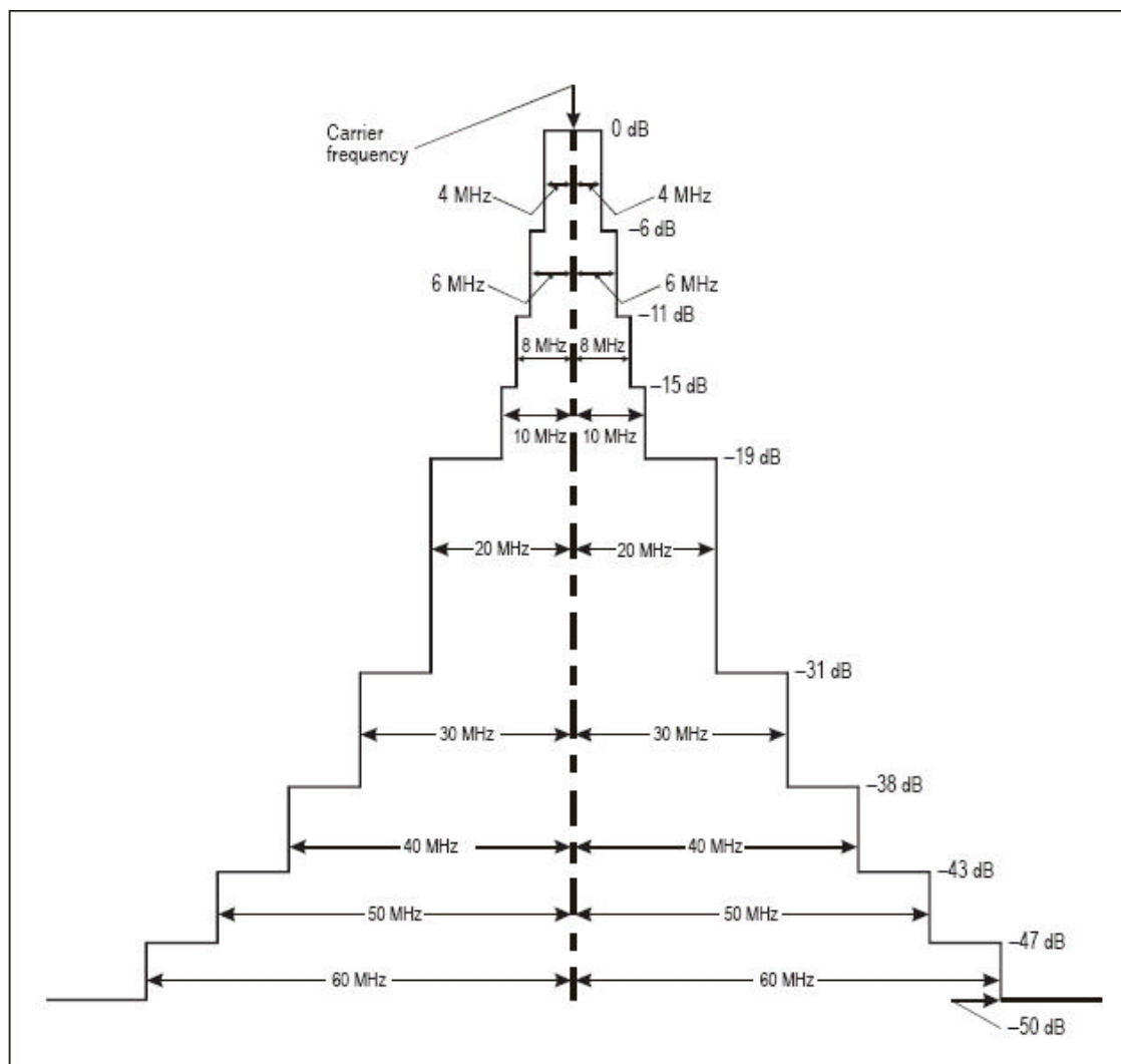
Figure 3-2. Required spectrum limits for interrogator transmitter
