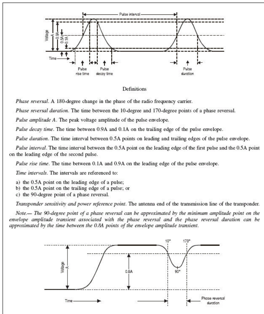
Figure 3-1. Definitions of secondary surveillance radar waveform shapes, intervals and the reference point for sensitivity and power
