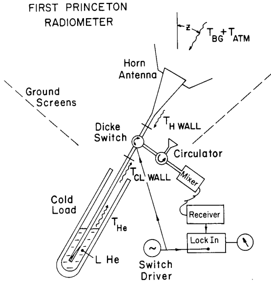
Fig. 2. The Princeton 3 cm radiometer. The switch connections could be reversed to measure and remove its offset.
