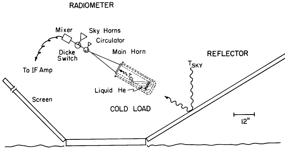
Fig. 3. The method used for three radiometers, \lambda = 3.2, 1.58 and 0.86 cm. The results fit a blackbody spectrum and gave a radiation temperature of 2.68 + 0.09 - 0.14 K.
