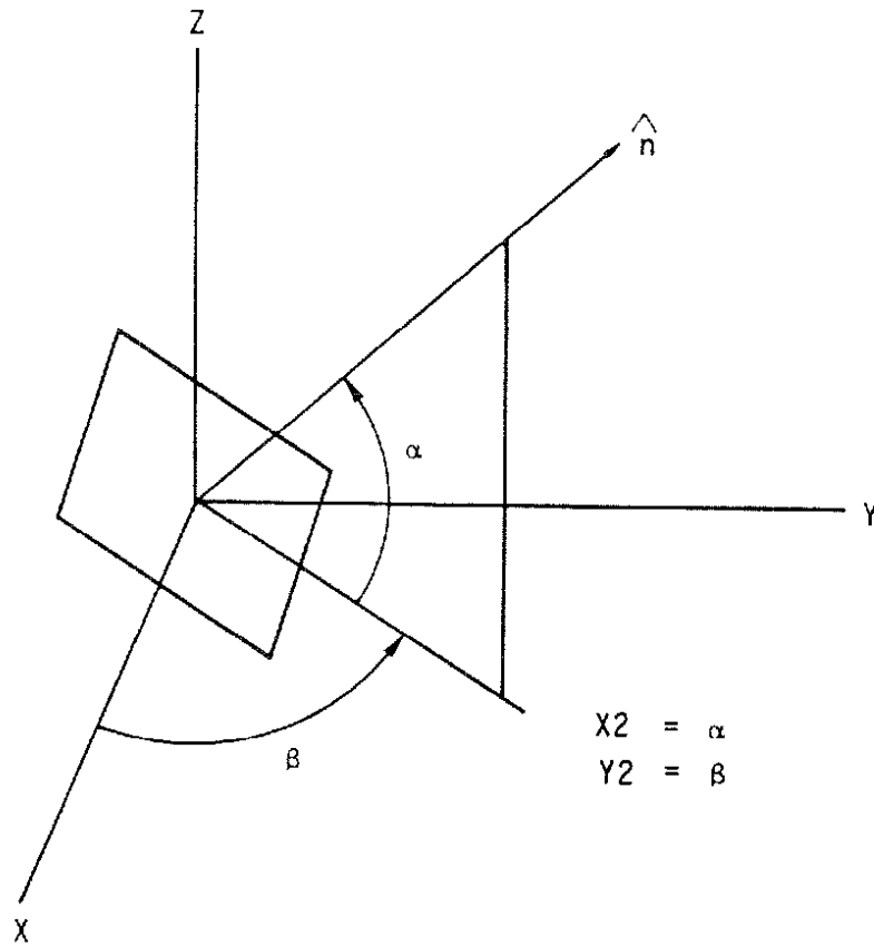
(a) Arbitrary Patch Shape (NS = 0)
