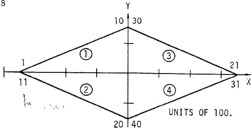
Figure 8. Rhombic Antenna - 2 Planes of Symmetry.
