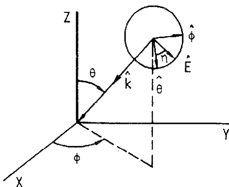
Figure 14. Specification of Incident Wave.
