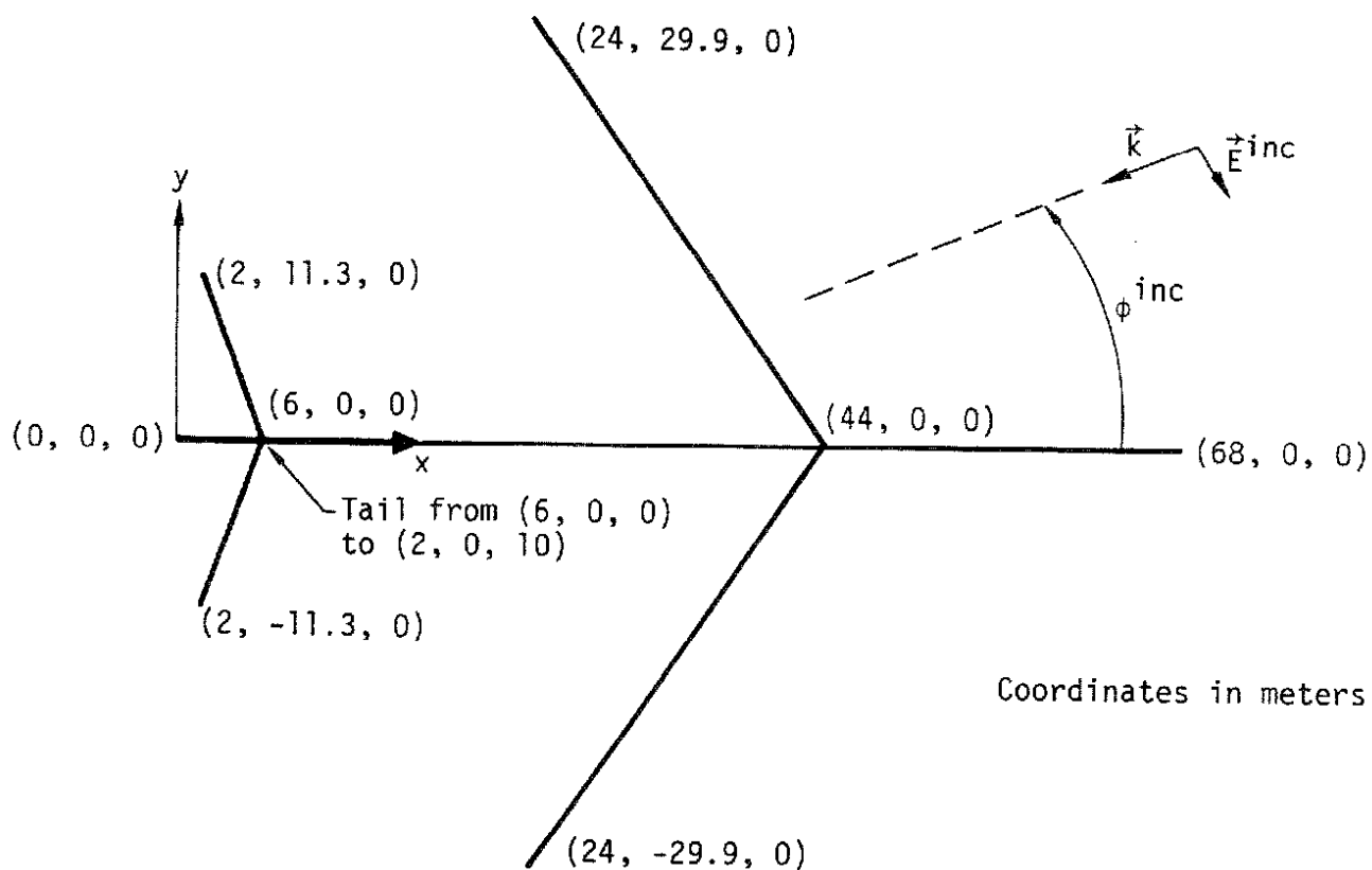
Figure 19. Stick model of aircraft.
