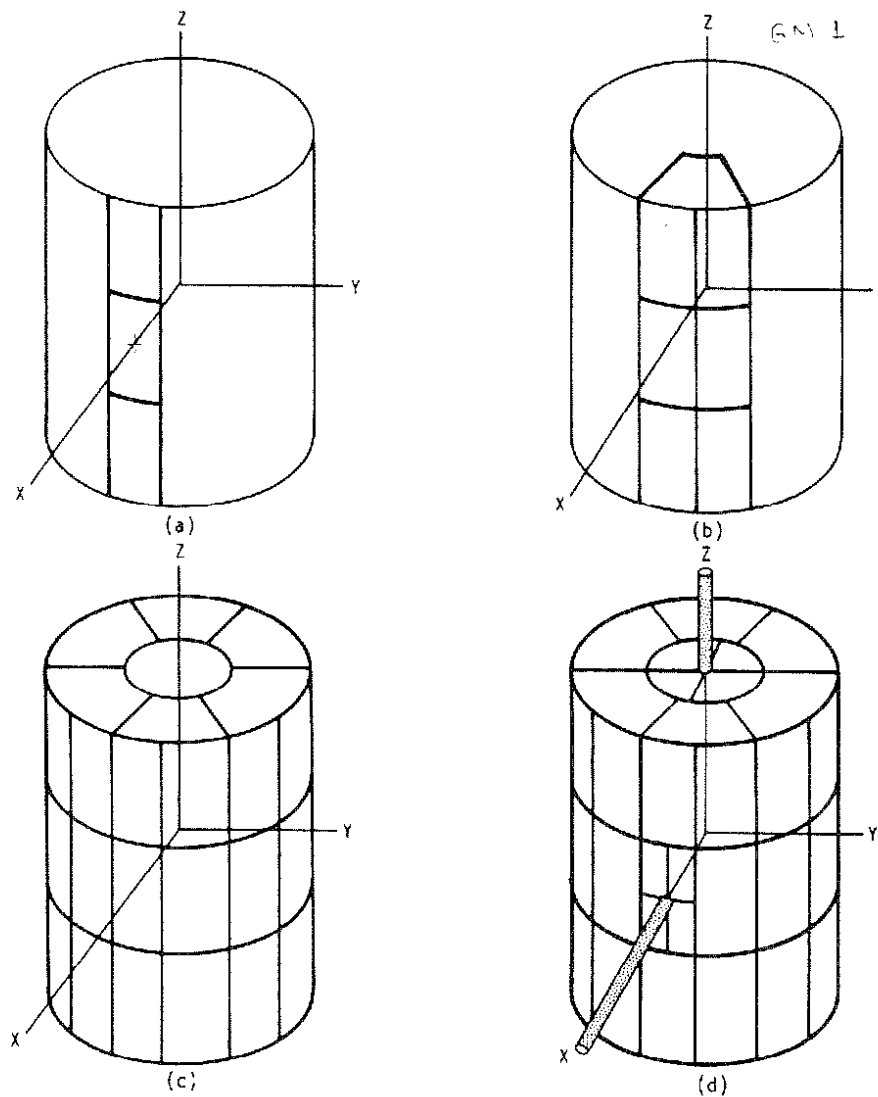
Figure 12. Development of Surface Model for Cylinder with Attached Wires.
