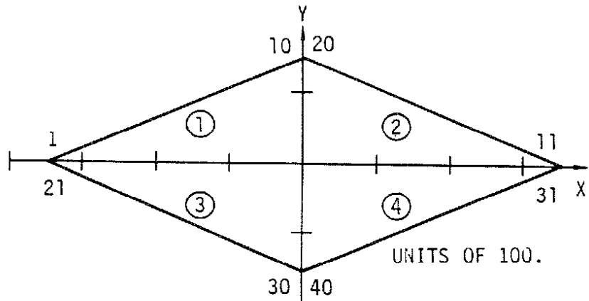
Figure 9. Rhombic Antenna - 1 Plane of Symmetry.
