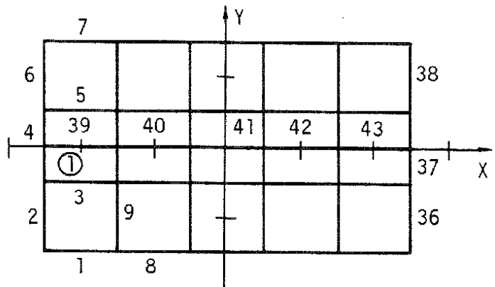
Figure 11. Wire Grid Plate and Dipole.
