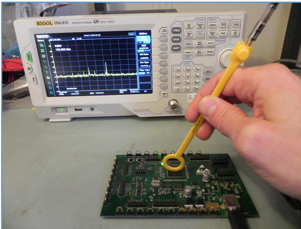
Figure 7-4: An example of using an H-field probe and spectrum analyzer to find trouble spots on a board. Note the orientation of the H-field probe
