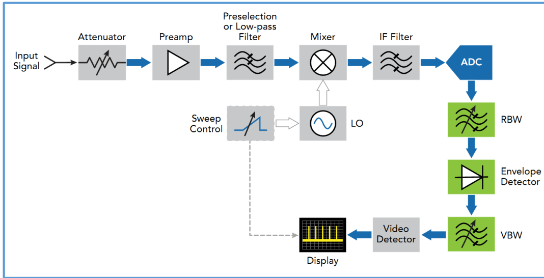
Figure 3-15: Block diagram of a swept superheterodyne design showing the location of the final stage of filtering and detector (RBW, Envelope, and VBW).
