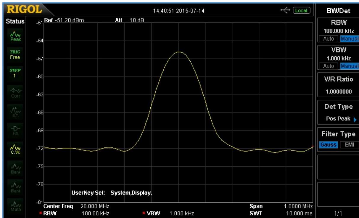
Figure 3-26: Identical 20MHz signal with the VBW decreased to 1kHz. Note smoothing of the trace. Note that decreasing the VBW setting can increase the sweep time.
