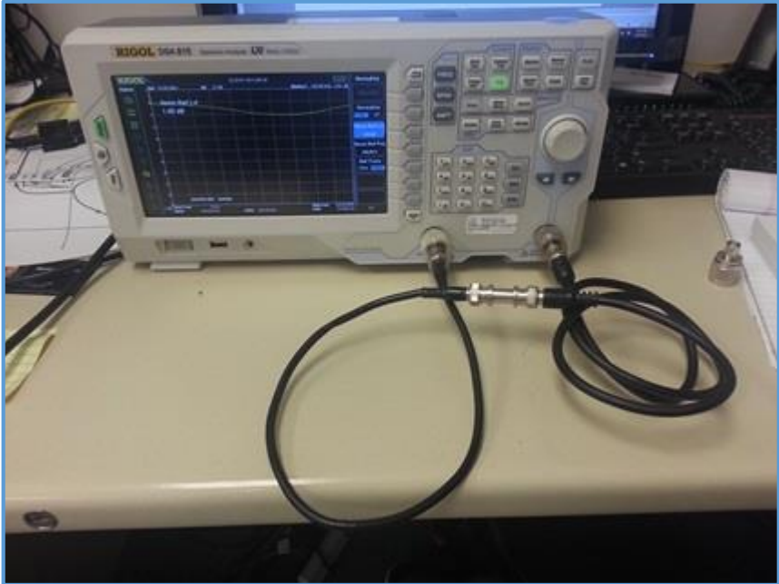
Figure 4-11: Cable-under-test connected.
