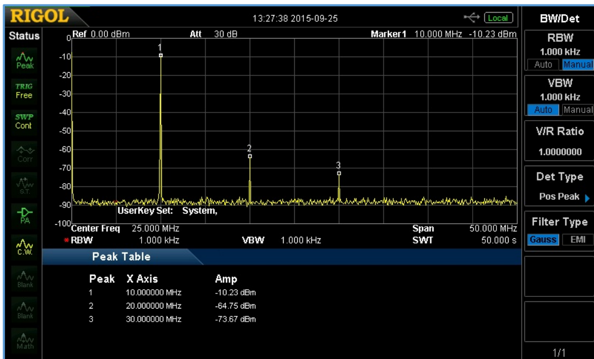
Figure 5-12: 10MHz sine input into a spectrum analyzer. Note 1 st and 2 nd harmonics.
