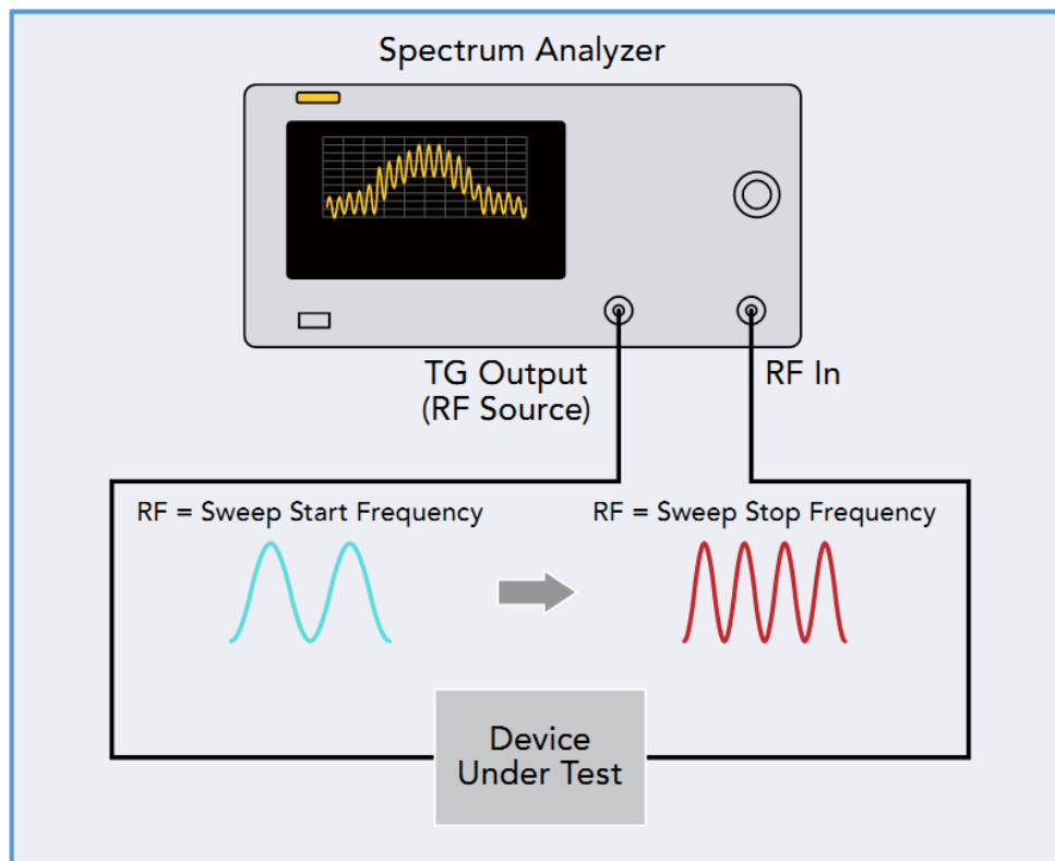
Figure 4-1: Example of a spectrum analyzer with tracking generator sweeping a DUT.
