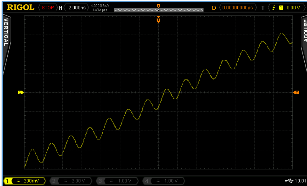
Figure 7-17: Zoomed data to show details.
