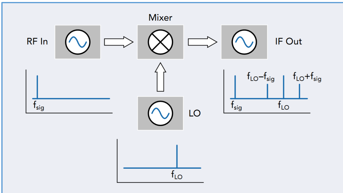
Figure 3-7: The input signal ( f_{sig} ) is mixed with the local oscillator signal ( f_{LO} ). The result is the f_{out} , which includes the fundamental mixed products.
