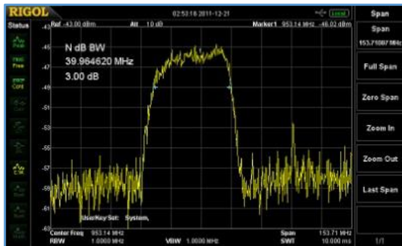
Figure 4-4: After Auto.
